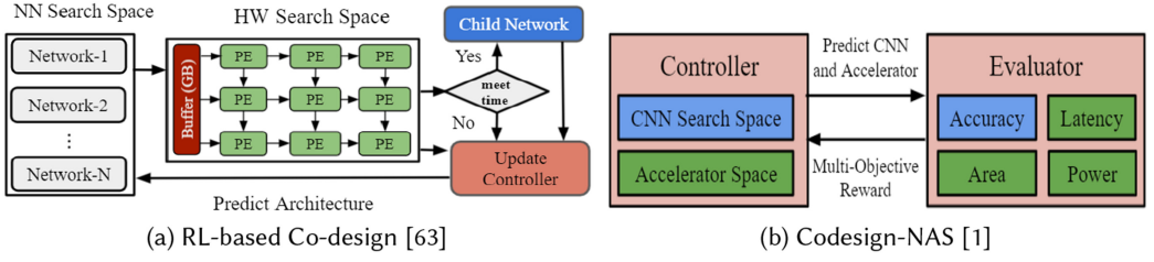
Fig. 12. Reinforcement learning-based network and accelerator architecture co-search methods.
