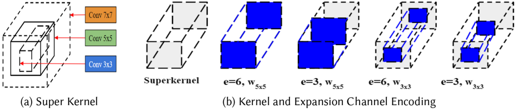
Fig. 8. Single Path NAS [116].
